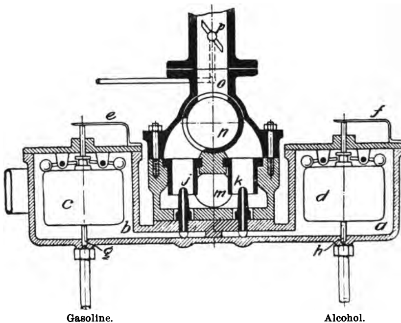
FIG. 30.—Alcohol Carbureter.
